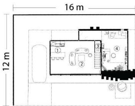
PLAN FLOOR 01
